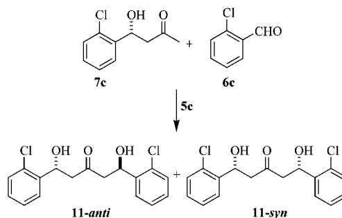
Scheme 3. Reaction of aldol product 7c with aldehyde 6c .
