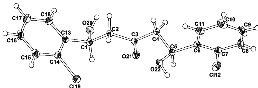
Figure 1. Crystal structure of anti - 11 .
