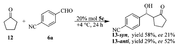
Scheme 4. Reaction of cyclopentanone ( 12 ) with 4-cyanobenzaldehyde ( 6a ).
