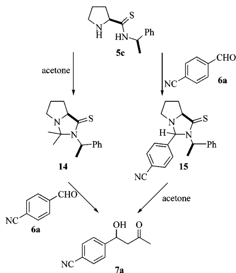
Scheme 6. Reactions of 5c with acetone and aldehyde 6a .
