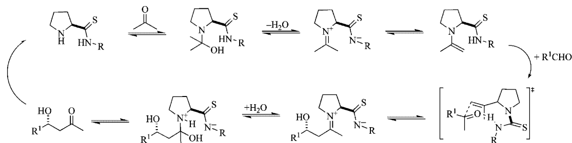
Scheme 5. Proposed mechanism for aldol reactions catalysed by 5 .
