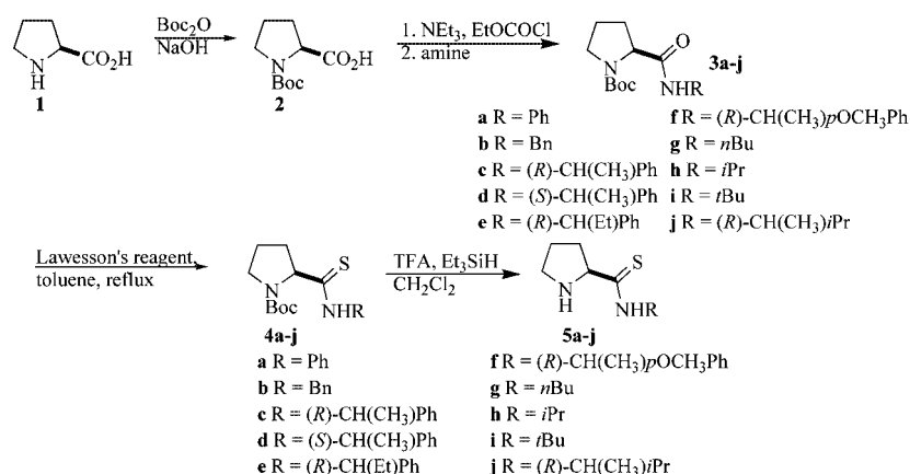
Scheme 1. Synthesis of L-prolinethioamides.
