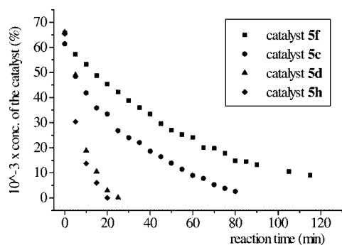
Figure 3. Graph showing the conversion of catalysts into imidazolidinethiones of type 14 as a function of time.
