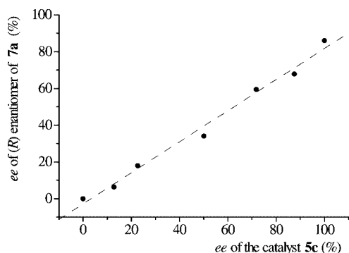
Figure 2. Linear effect in the aldol reaction of acetone with 4-cyanobenzaldehyde ( 6a ).
